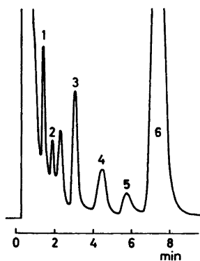
Fig. 1. Gas chromatographic separation on QF-1 at 120 °C of the dicarboxylic acids as Me 3 Si derivatives. Identified acids: 1. Oxalic. 2. C -Methyltartronic. 3. Tartronic. 4. Deoxytetra- and C -(hydroxymethyl)tartronic. 5. O -Methylerythric. 6. C -(2-Hydroxyethyl)tartronic.
