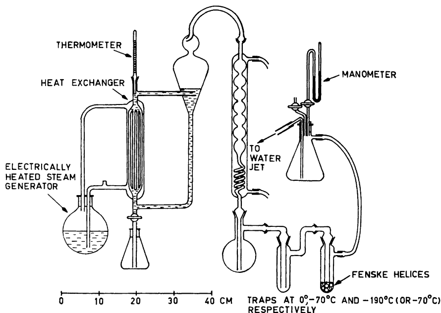
Fig. 1. Diagram of the distillation apparatus.
