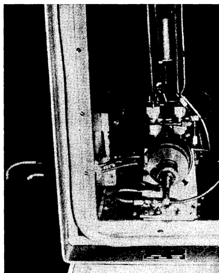
Fig. 5. Photograph showing the location of the sample inlet valve in the gas chromatography apparatus.
