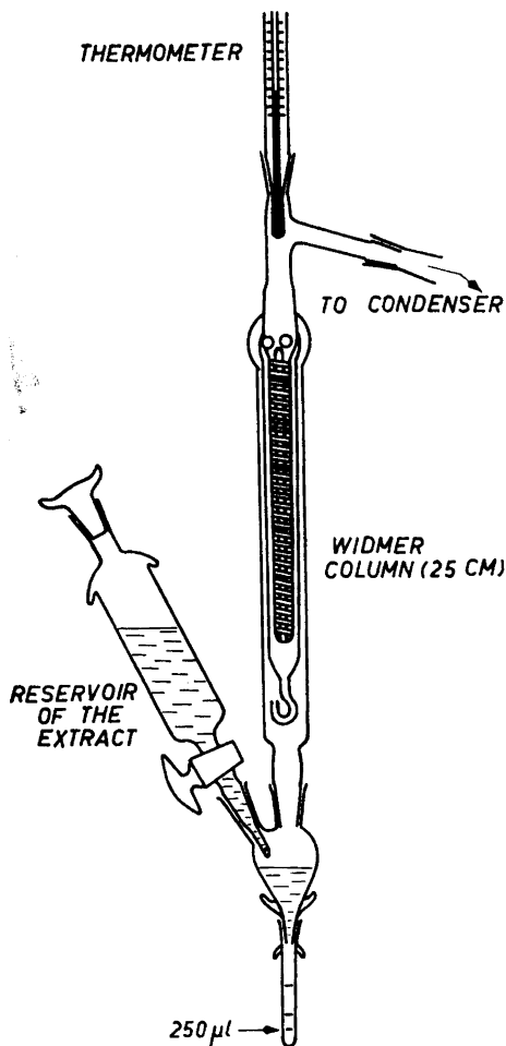
Fig. 3. A Widmer column distillation apparatus for the concentration of the flavour extract. The detachable and graduated tube at the lower end of the apparatus is placed in a thermostat (30°C or 60°C for ethyl chloride and pentane-ether, respectively) and closed with a Teflon stopper when the desired final volume has been reached.
