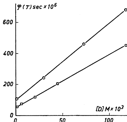
Fig. 5. \varphi(\tau) = \tau_{\text{corr}}/(1 - K \tau_{\text{corr}}) vs. biacetyl concentration [D]. Data from Table 2. \square Series 1, K = 3280 \text{ sec}^{-1} . \circ Series 2, K = 2353 \text{ sec}^{-1} . For further explanations see text.
