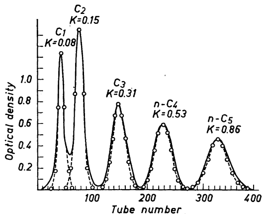
Fig. 1. Distribution of 2,4-dinitrophenylhydrazones of normal aliphatic aldehydes (C 1 –C 5 ) in the solvent system: petroleum ether: ethylene glycol monomethyl ether: water, (10:10:2.5). — experimental curve, optical density of the bottom phase at 360 m \mu . O—O theoretical curve.
