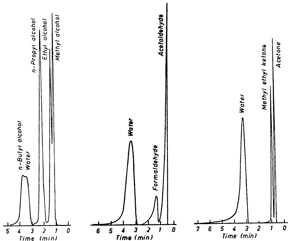
Fig. 1. Water-alcohol mixture. Column No. 1. Temperature 100°C. Flow of He 50 ml/min.
